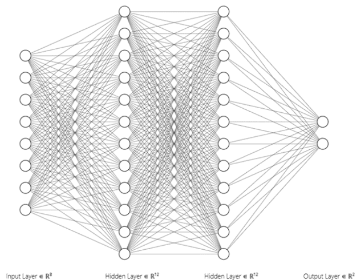
Figure 3. Neural Network
